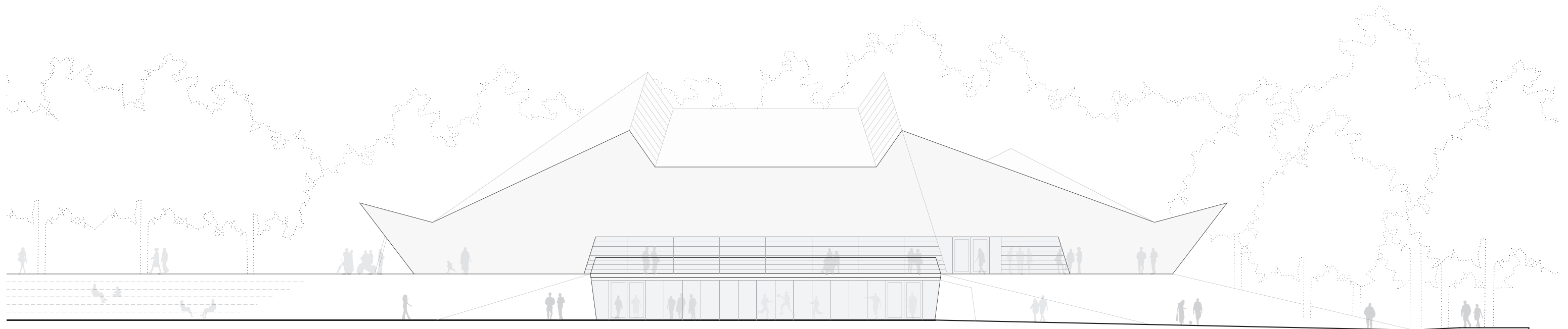
South Elevation
